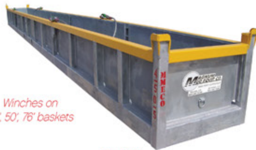
4' x 50' EMPTY WEIGHT: 9,200 lbs. MAX GROSS WEIGHT: 40,000 lbs. (4' x 76' Not shown)
